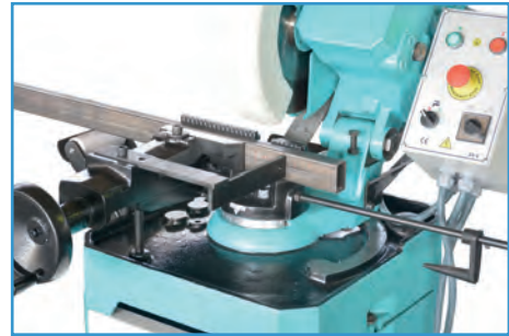
T tipi Tekli Mengene T type Single Vice
