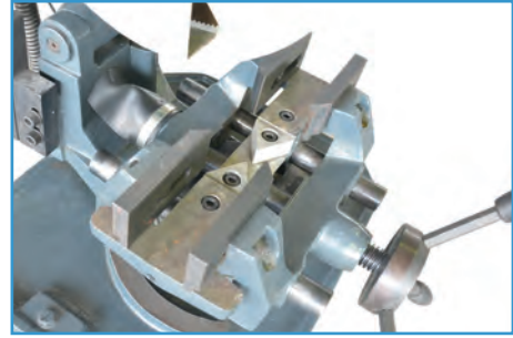
V Tipi Çift Mengene V type Double Vice
